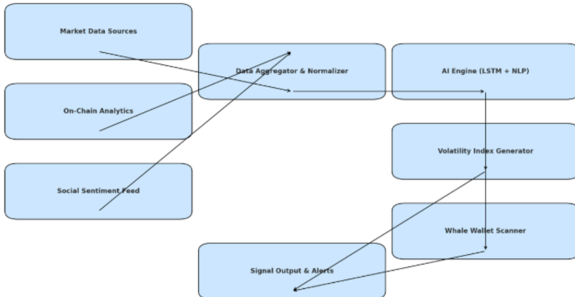
Pixiu AI Trading Platform - Functional Architecture
